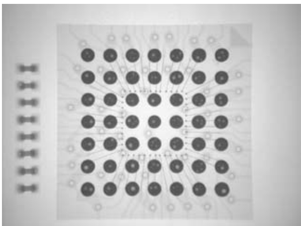
BGA X-ray Inspection
